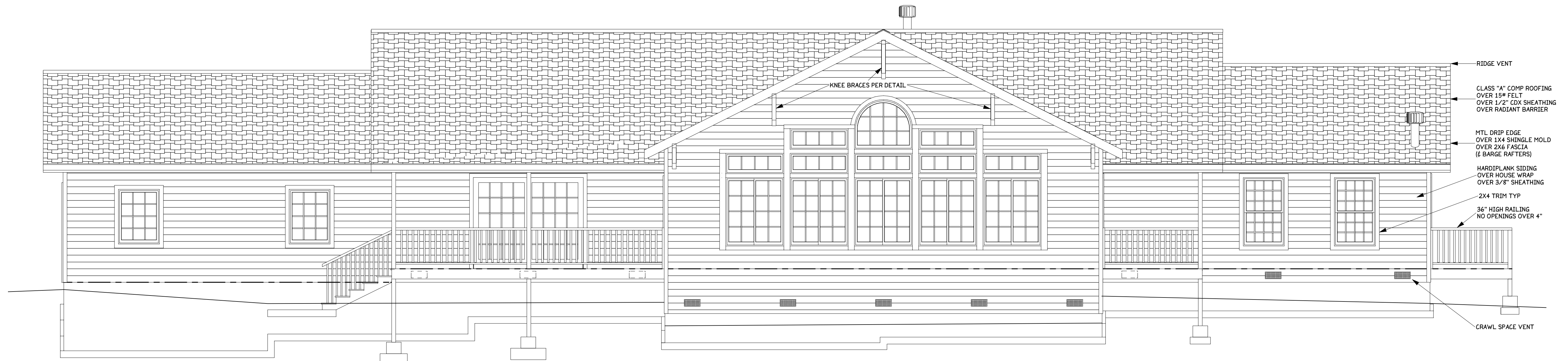
SOUTH (FRONT) ELEVATION SCALE: 1/4" = 1'
