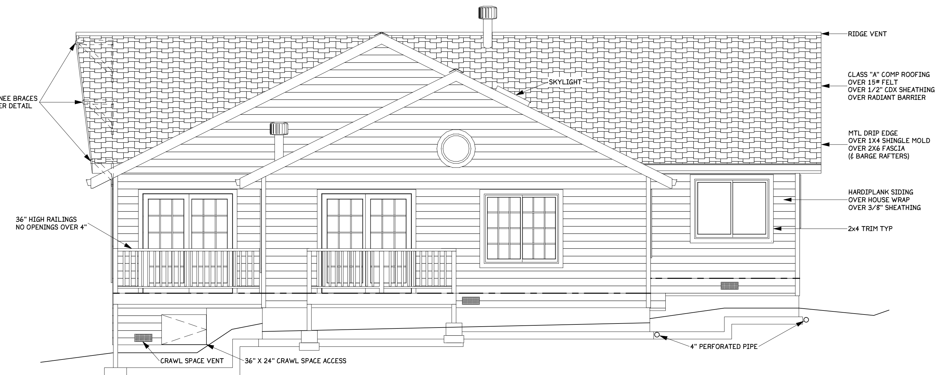
EAST (RIGHT) ELEVATION SCALE: 1/4" = 1'
