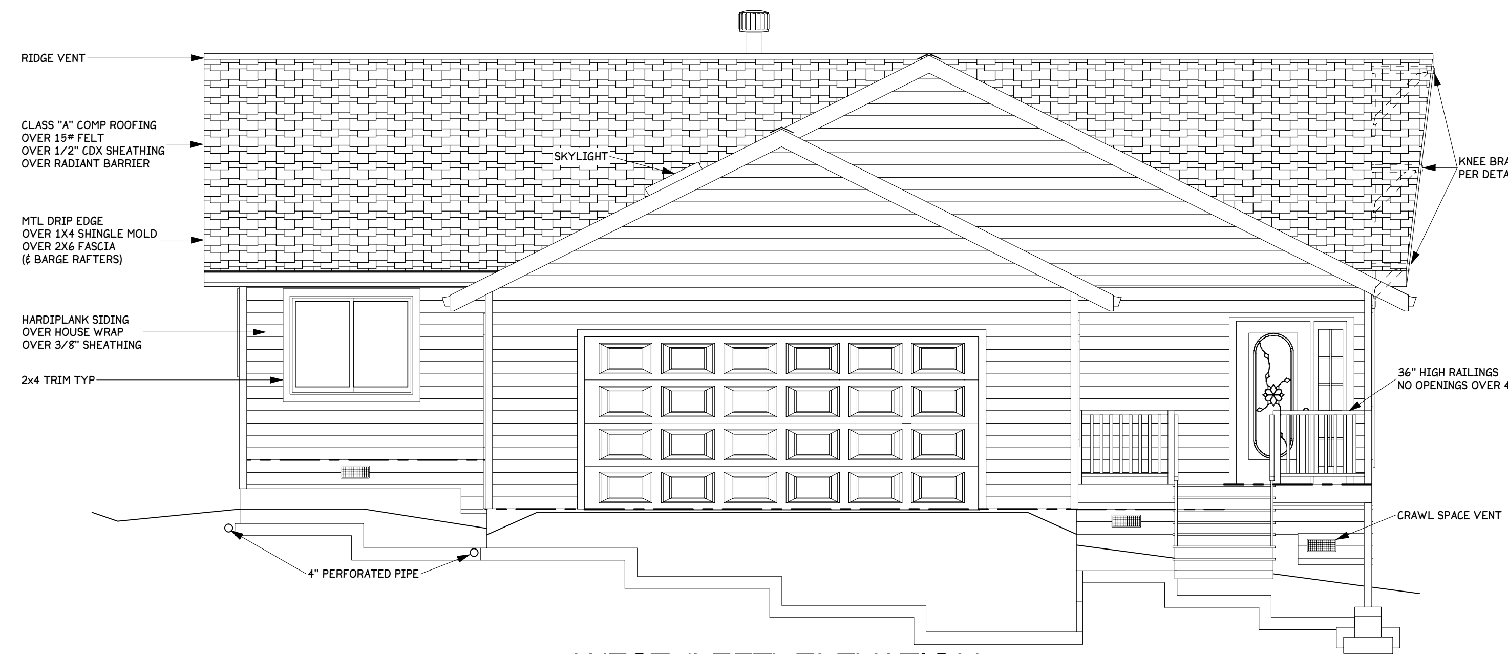
WEST (LEFT) ELEVATION SCALE: 1/4" = 1'
