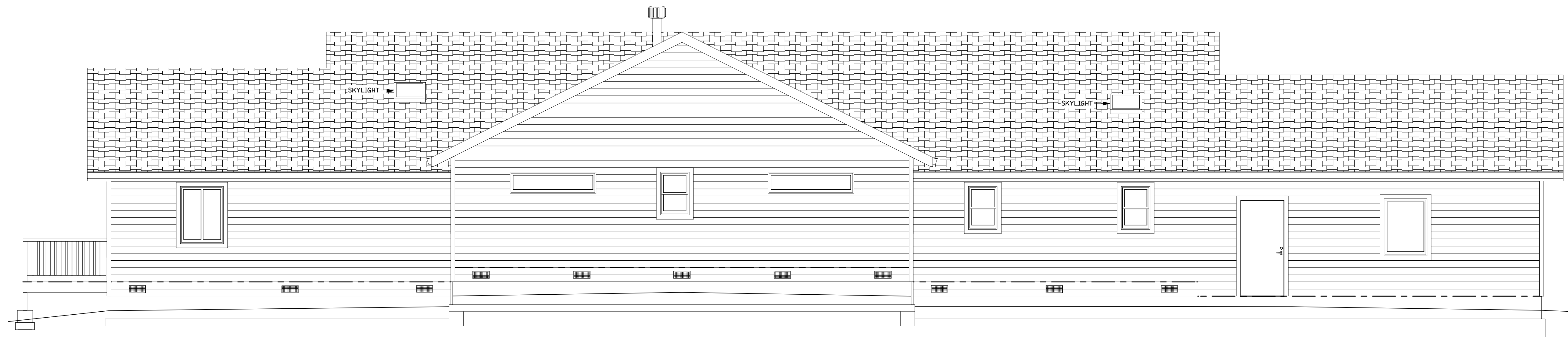
NORTH (BACK) ELEVATION SCALE: 1/4" = 1'
